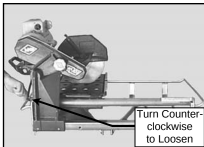
(E) Loosen front and rear Guide Bar Retaining Bolts
